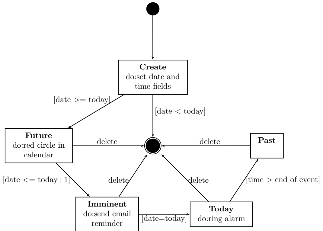
Figure 12.4: State machine for the class Event
